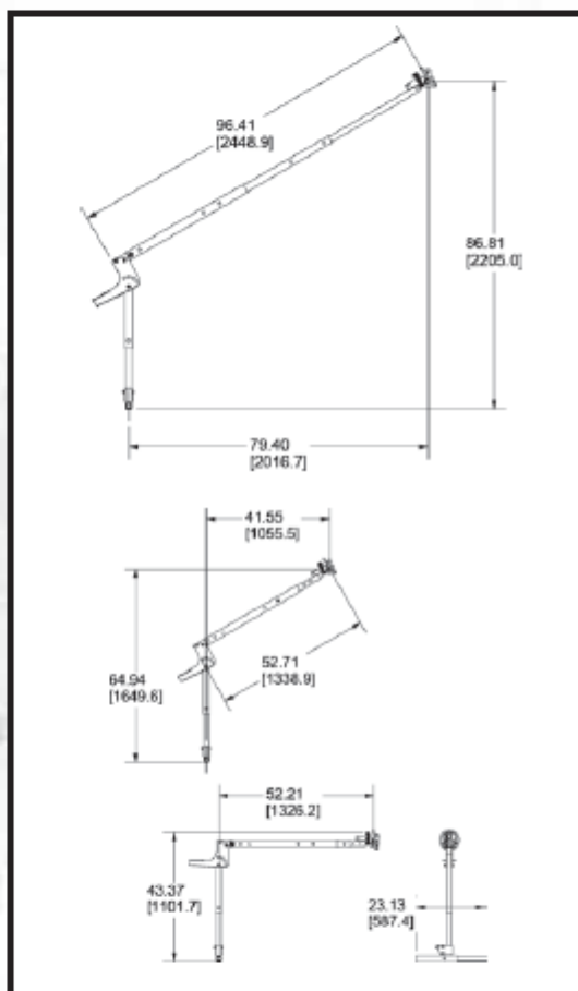
Pro-2 Pole Hoist
