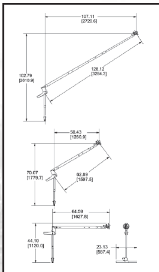
Pro-1 Pole Hoist
