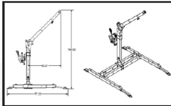
PT# 20080; Pro-3 HD Hoist System 42" Offset (Max)
